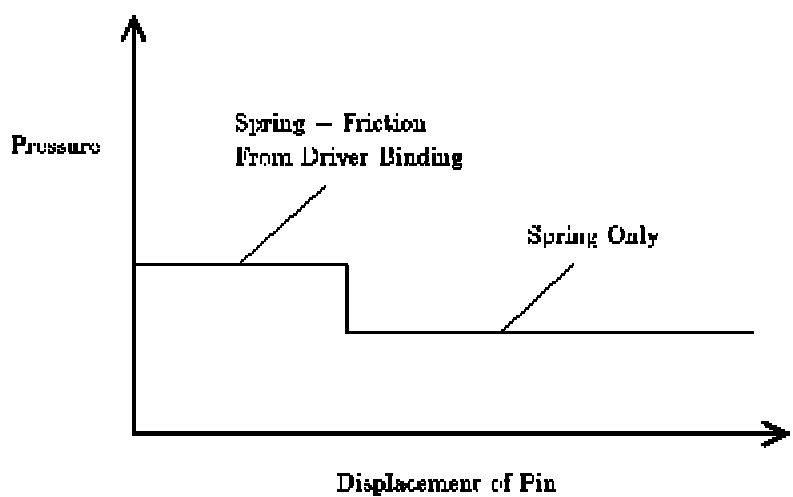
Figure 9.3: Driver pin wider than key pin
