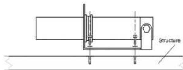
Figure 35: Sensor Mounting
